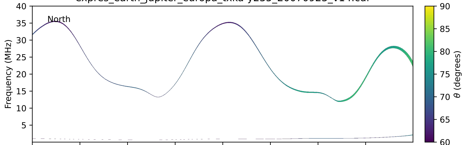
expres_earth_jupiter_europa_txka-y235_20070923_v14.cdf
