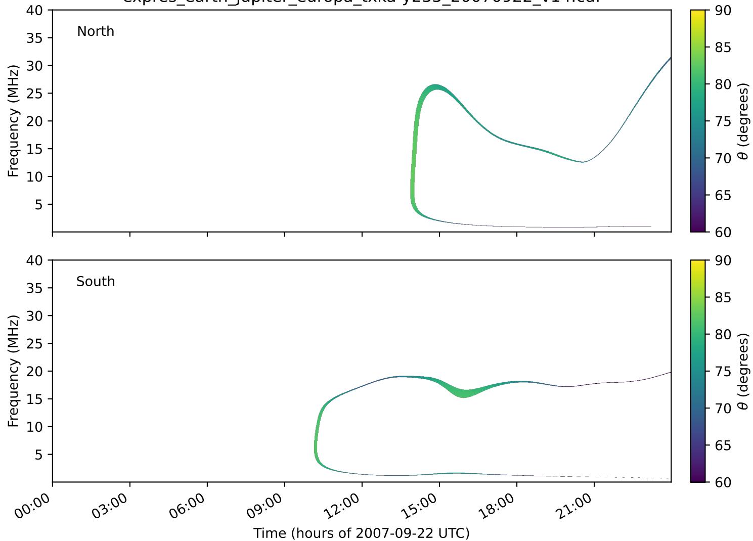
expres_earth_jupiter_europa_txka-y235_20070922_v14.cdf
