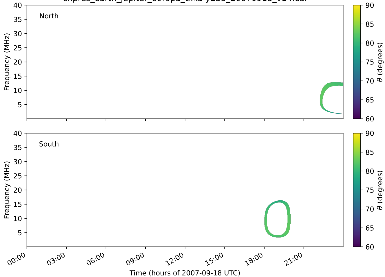
expres_earth_jupiter_europa_txka-y235_20070918_v14.cdf
