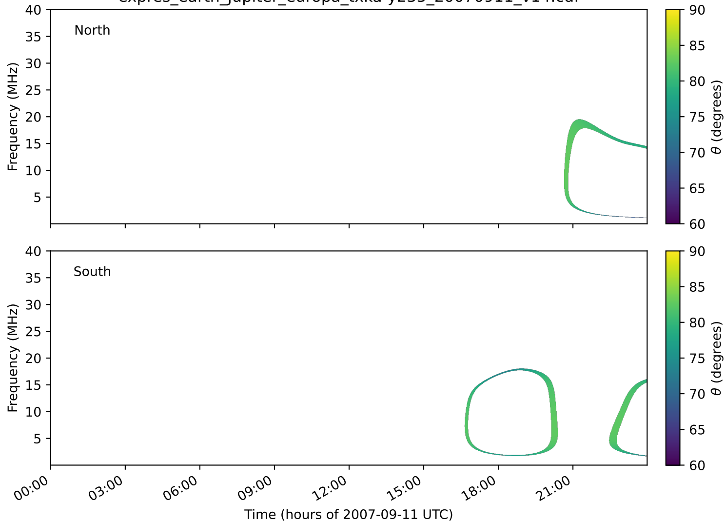
expres_earth_jupiter_europa_txka-y235_20070911_v14.cdf
