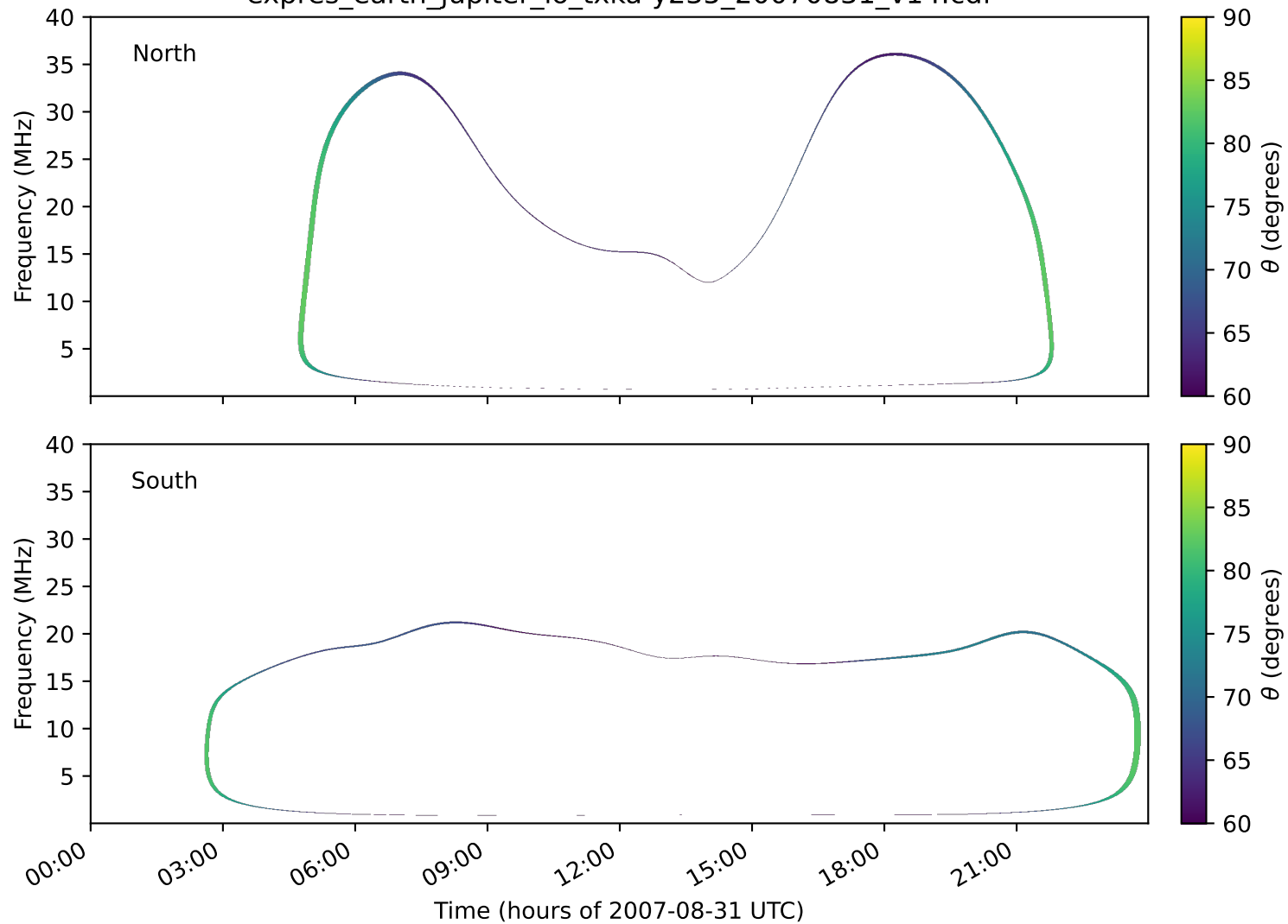
expres_earth_jupiter_io_txka-y235_20070831_v14.cdf
