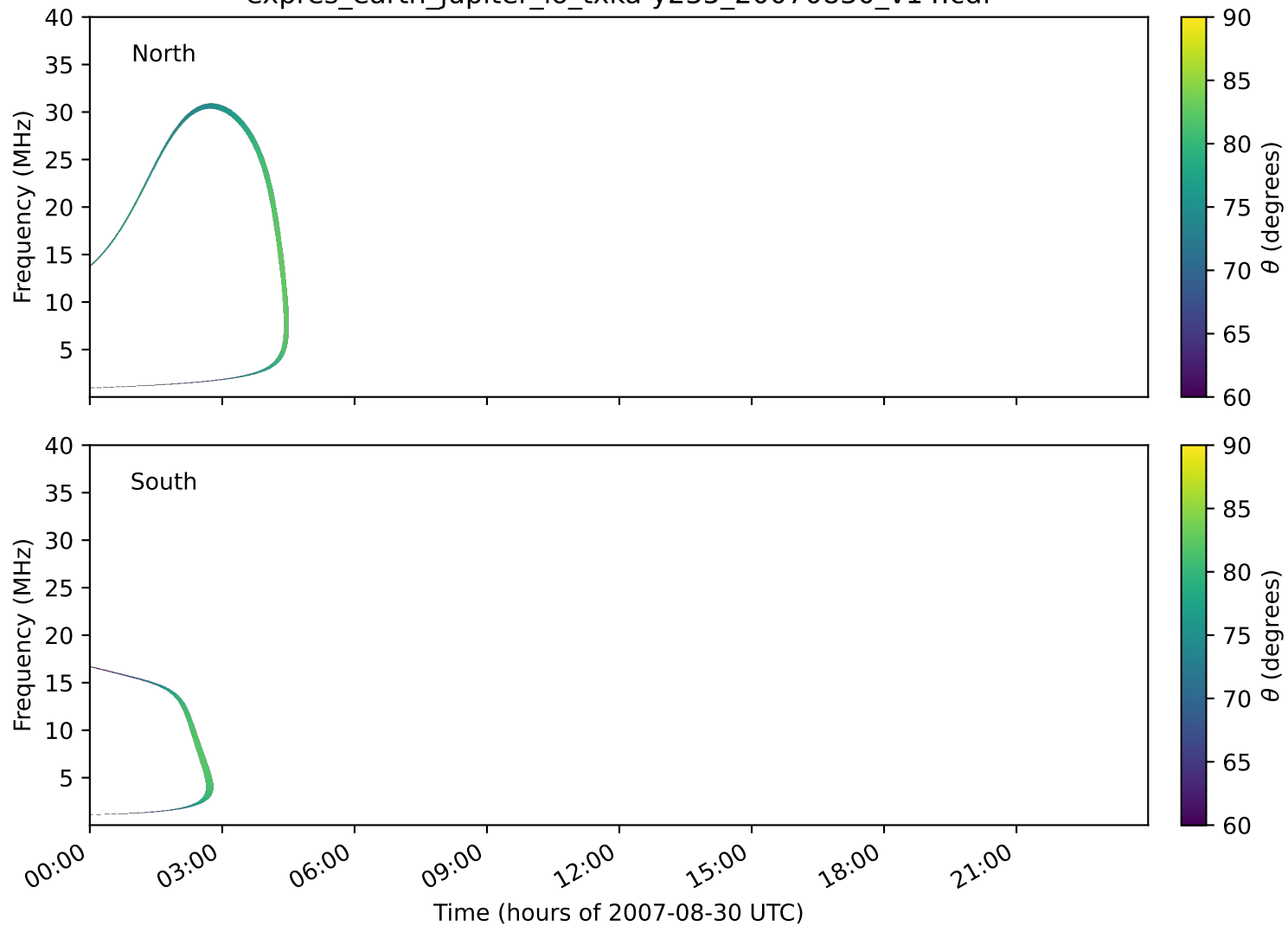
expres_earth_jupiter_io_txka-y235_20070830_v14.cdf
