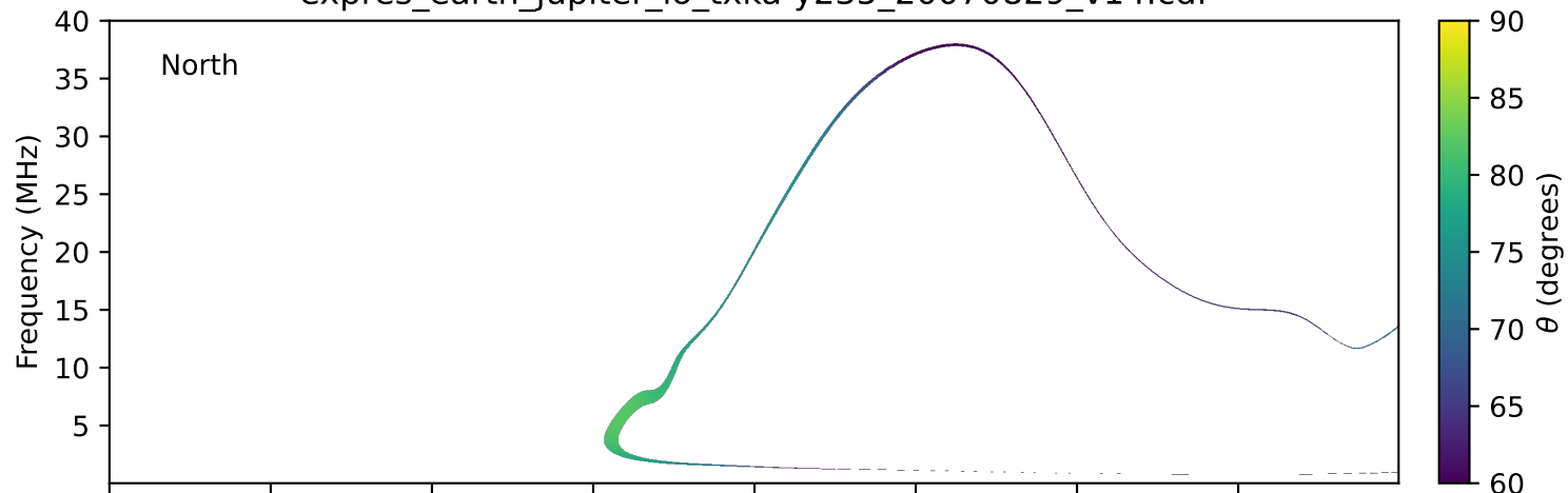
expres_earth_jupiter_io_txka-y235_20070829_v14.cdf
