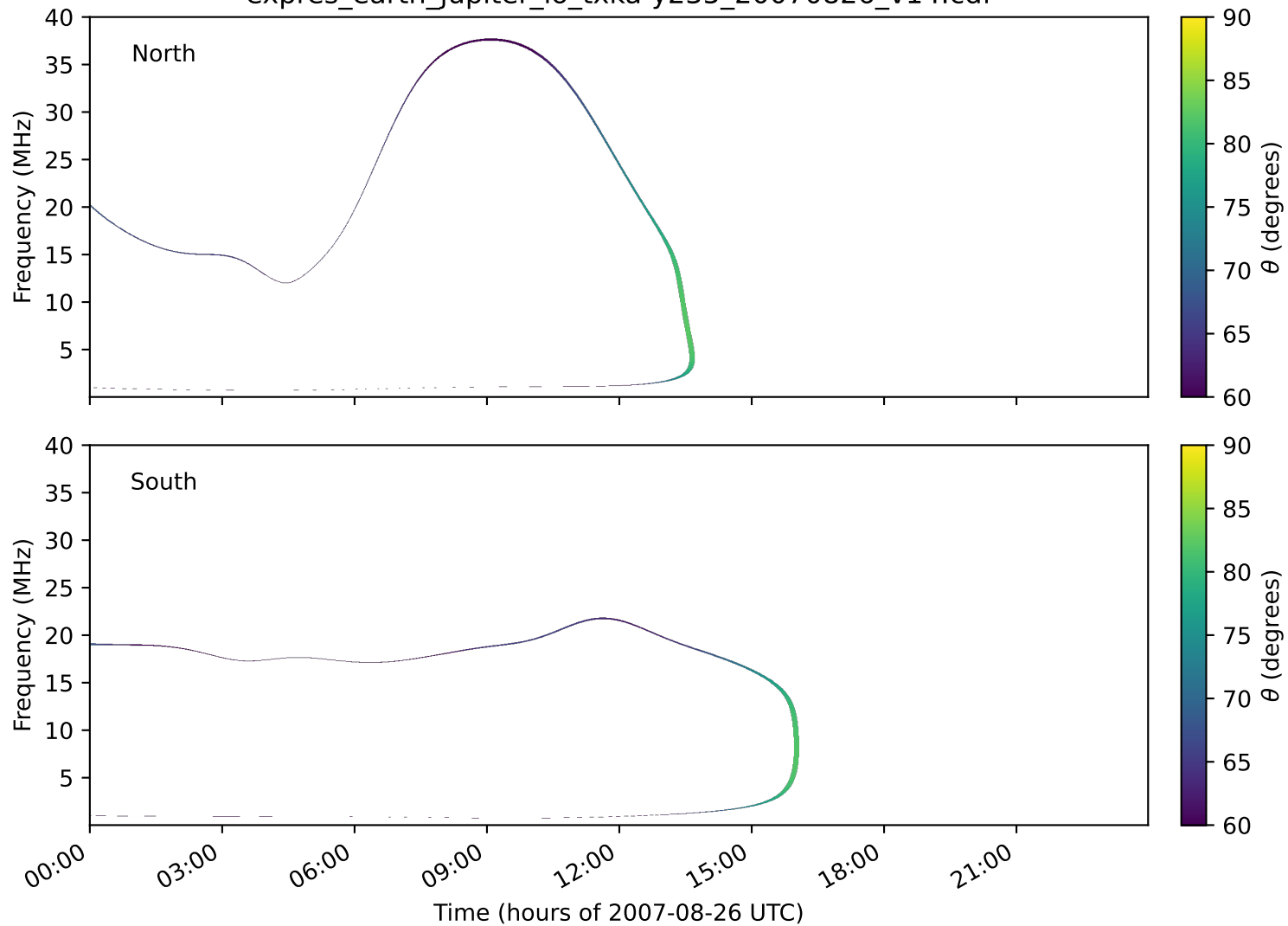
expres_earth_jupiter_io_txka-y235_20070826_v14.cdf
