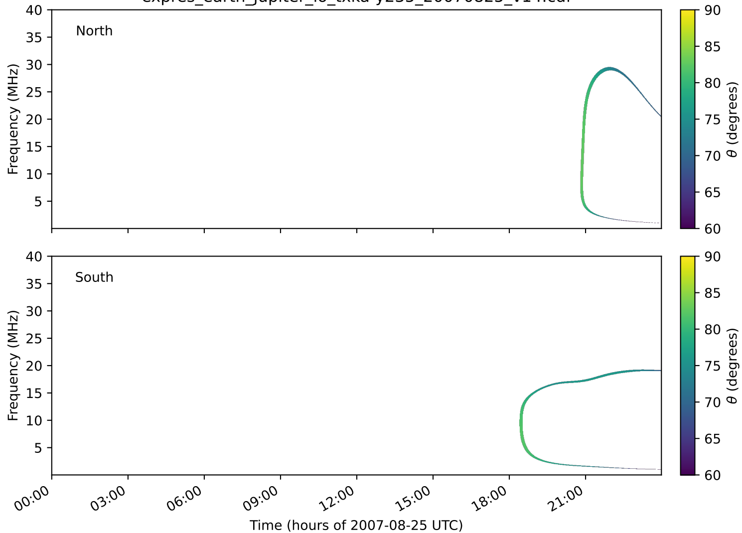
expres_earth_jupiter_io_txka-y235_20070825_v14.cdf
