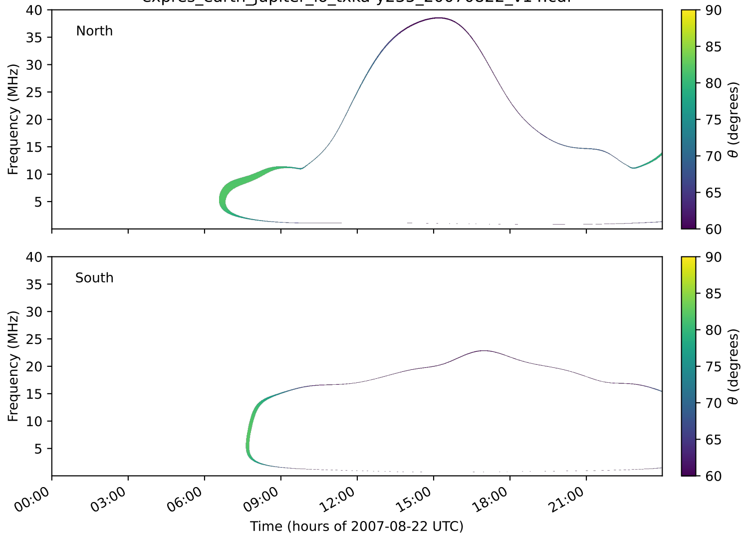
expres_earth_jupiter_io_txka-y235_20070822_v14.cdf
