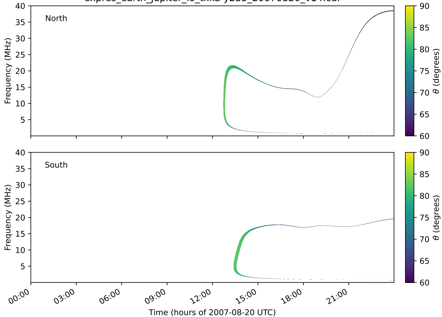
expres_earth_jupiter_io_txka-y235_20070820_v14.cdf
