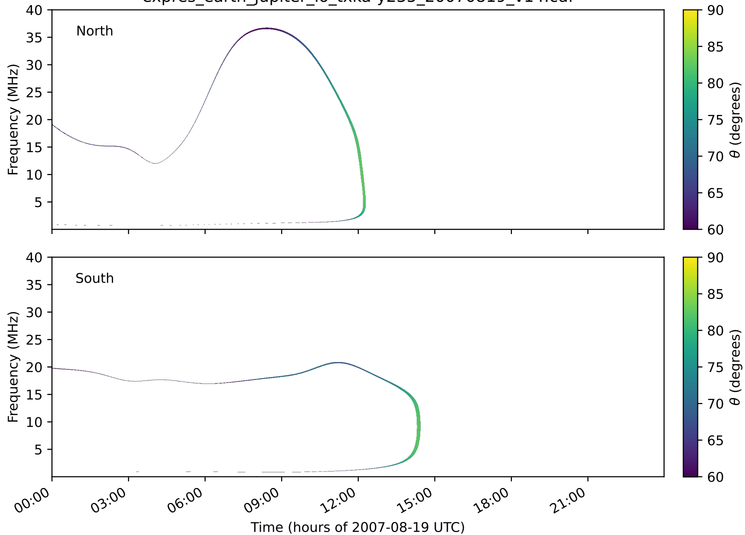
expres_earth_jupiter_io_txka-y235_20070819_v14.cdf
