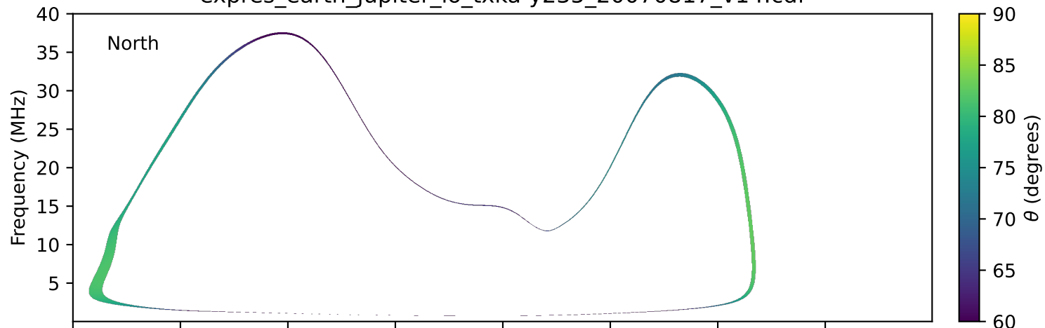
expres_earth_jupiter_io_txka-y235_20070817_v14.cdf
