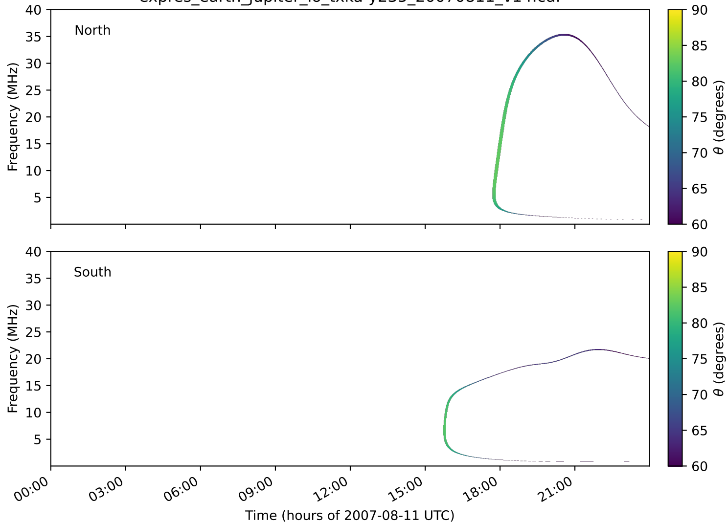
expres_earth_jupiter_io_txka-y235_20070811_v14.cdf
