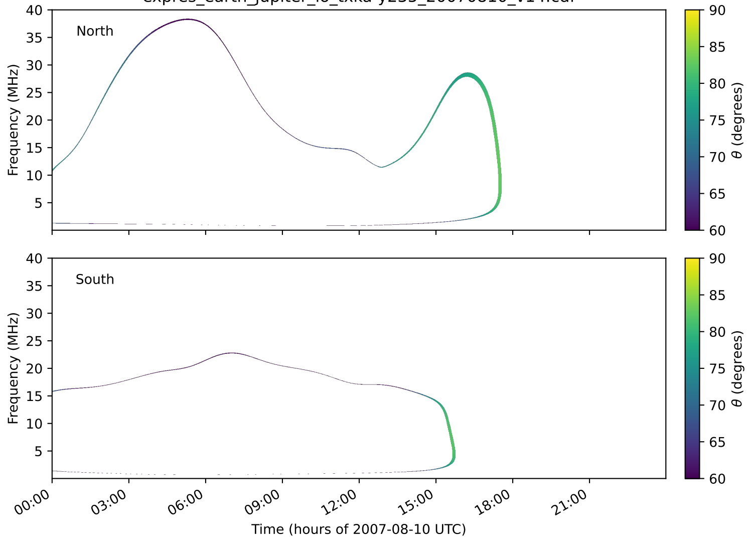
expres_earth_jupiter_io_txka-y235_20070810_v14.cdf
