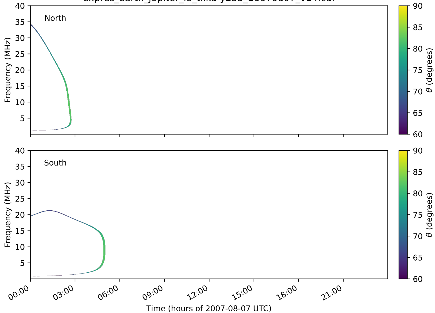
expres_earth_jupiter_io_txka-y235_20070807_v14.cdf
