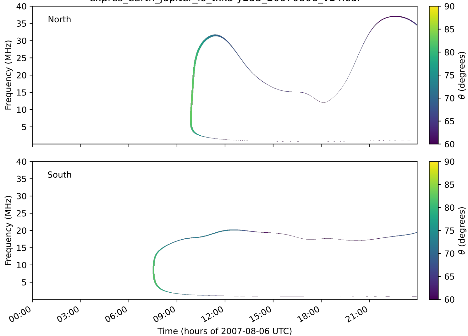
expres_earth_jupiter_io_txka-y235_20070806_v14.cdf
