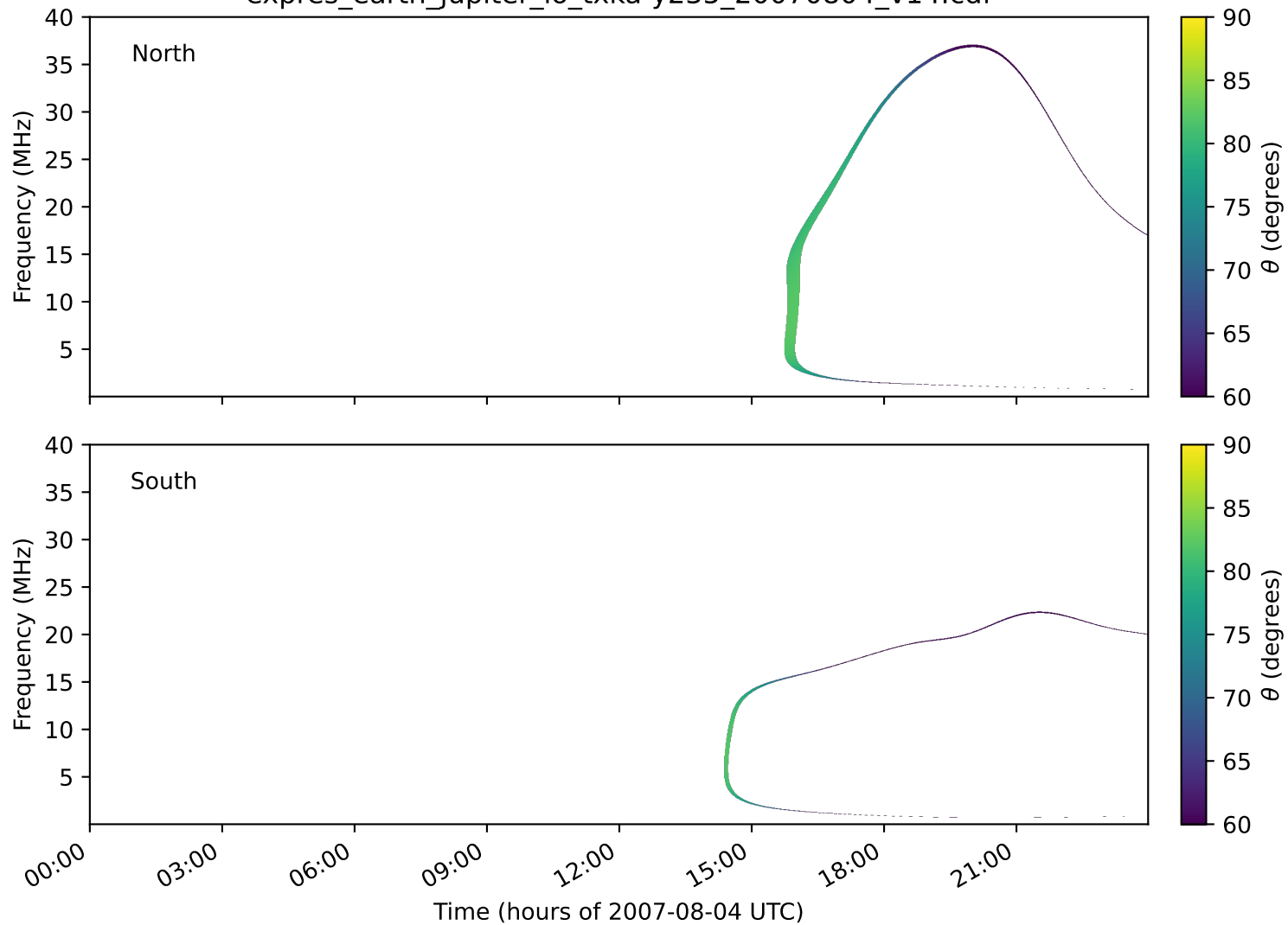
expres_earth_jupiter_io_txka-y235_20070804_v14.cdf
