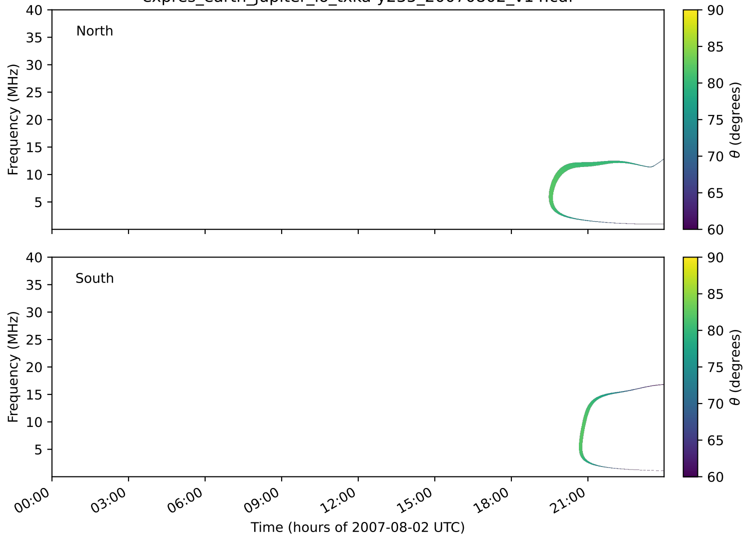
expres_earth_jupiter_io_txka-y235_20070802_v14.cdf
