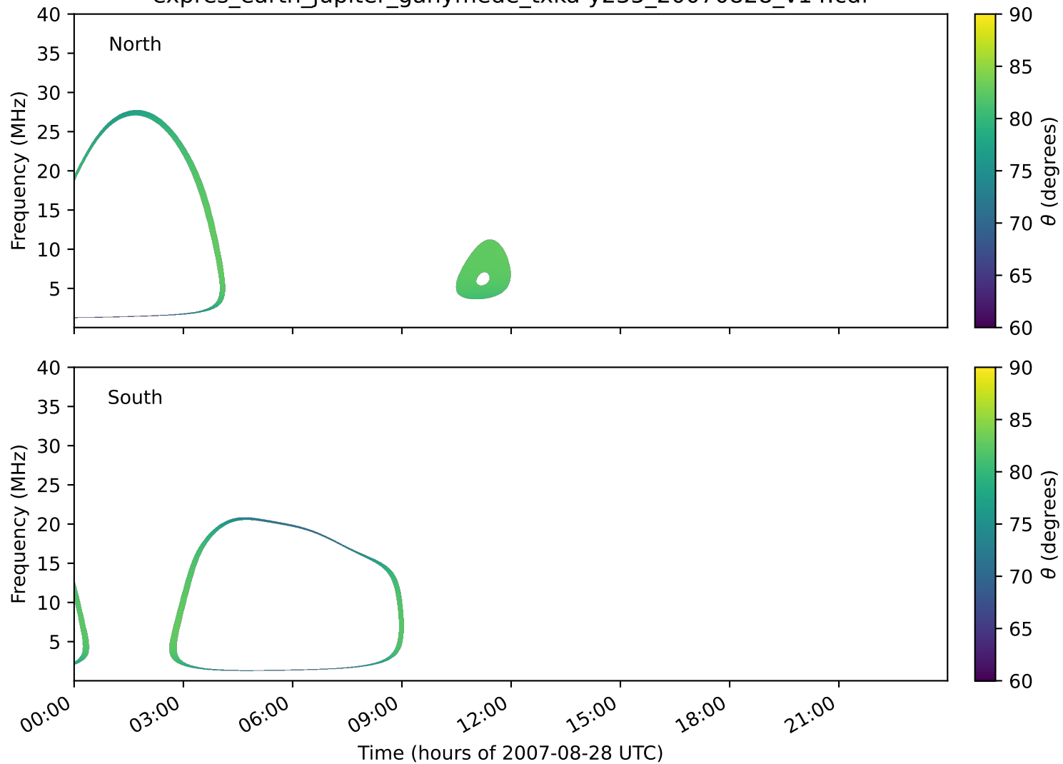
expres_earth_jupiter_ganymede_txka-y235_20070828_v14.cdf
