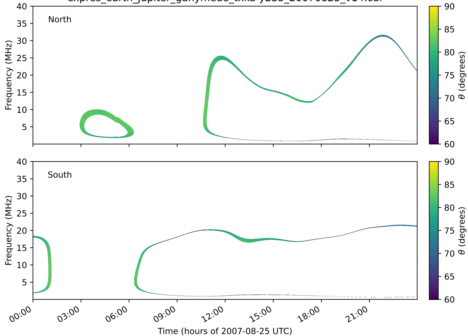
expres_earth_jupiter_ganymede_txka-y235_20070825_v14.cdf
