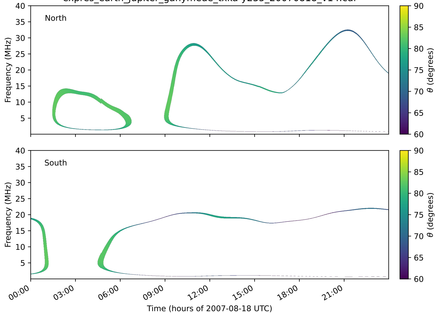
expres_earth_jupiter_ganymede_txka-y235_20070818_v14.cdf
