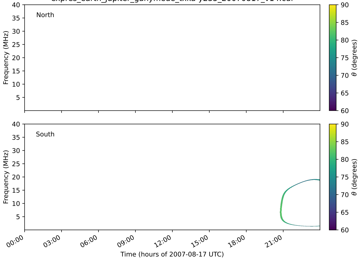
expres_earth_jupiter_ganymede_txka-y235_20070817_v14.cdf
