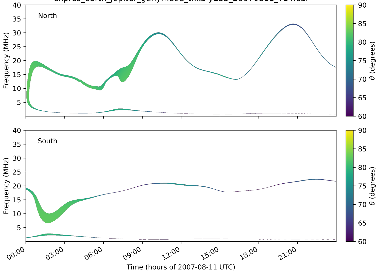
expres_earth_jupiter_ganymede_txka-y235_20070811_v14.cdf
