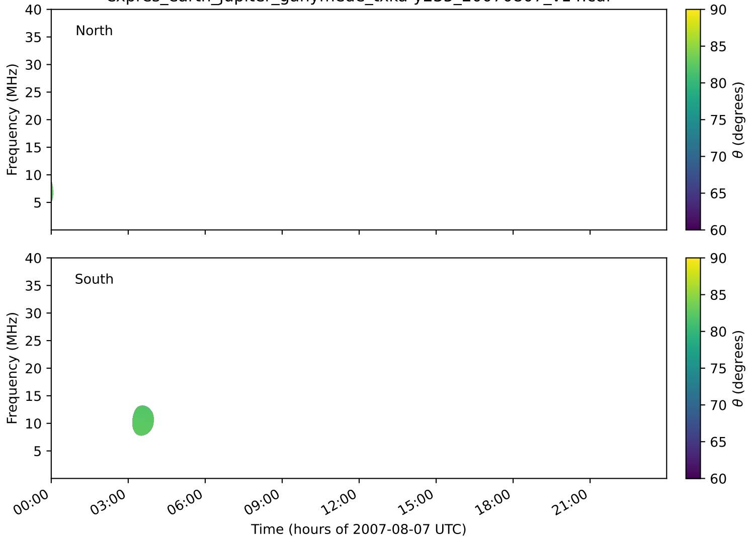
expres_earth_jupiter_ganymede_txka-y235_20070807_v14.cdf
