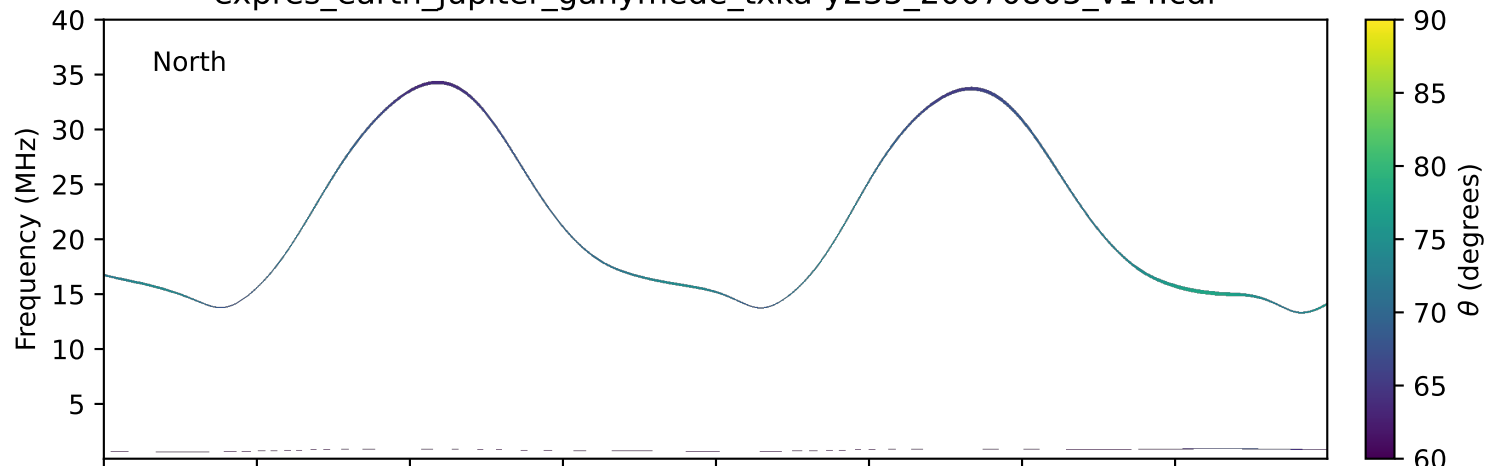
expres_earth_jupiter_ganymede_txka-y235_20070805_v14.cdf
