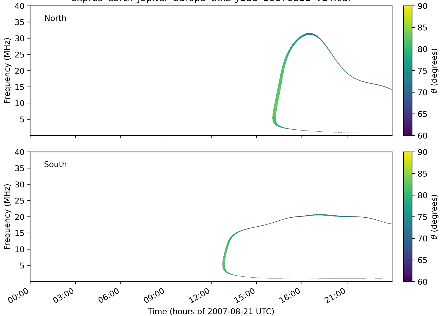
expres_earth_jupiter_europa_txka-y235_20070821_v14.cdf
