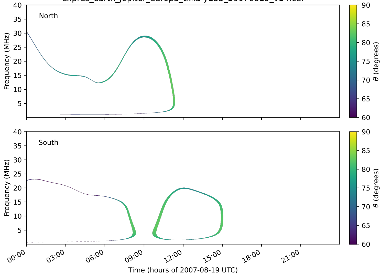
expres_earth_jupiter_europa_txka-y235_20070819_v14.cdf
