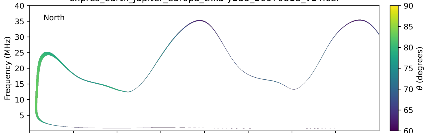
expres_earth_jupiter_europa_txka-y235_20070818_v14.cdf
