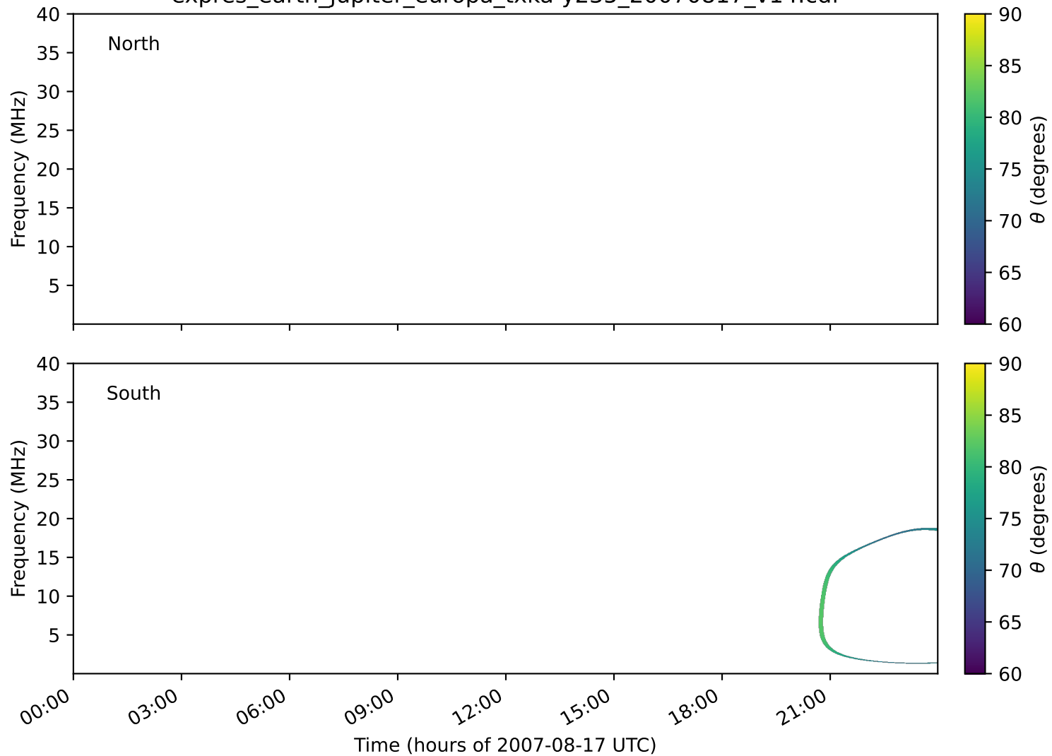
expres_earth_jupiter_europa_txka-y235_20070817_v14.cdf
