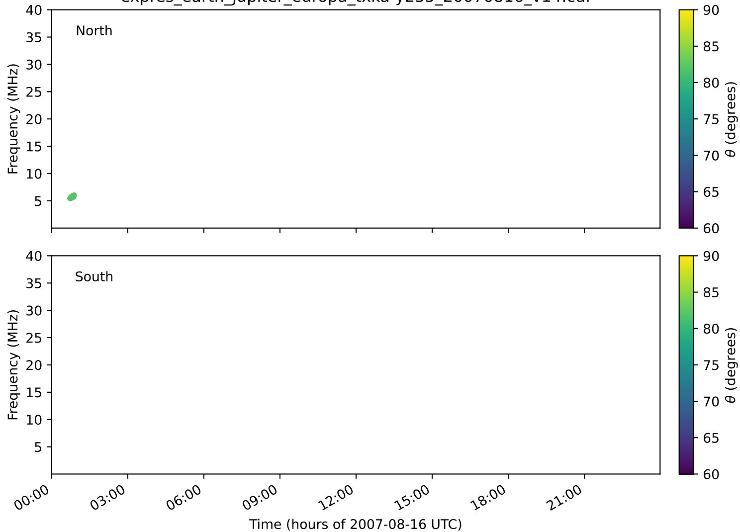
expres_earth_jupiter_europa_txka-y235_20070816_v14.cdf
