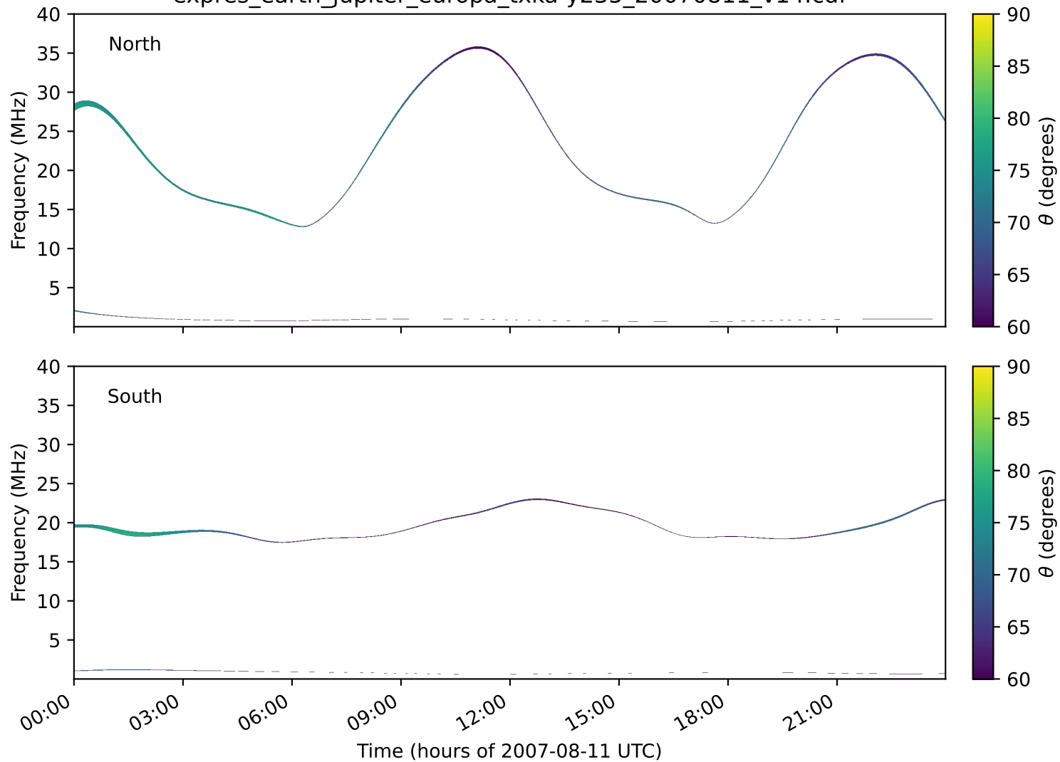
expres_earth_jupiter_europa_txka-y235_20070811_v14.cdf
