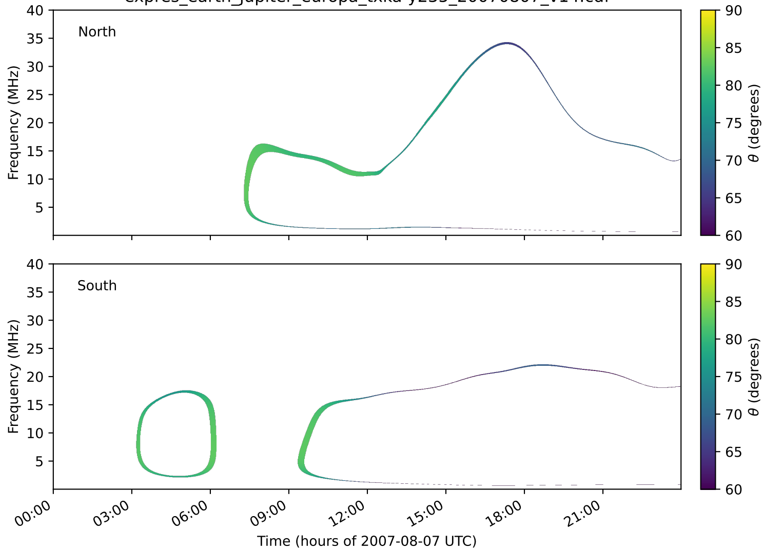
expres_earth_jupiter_europa_txka-y235_20070807_v14.cdf
