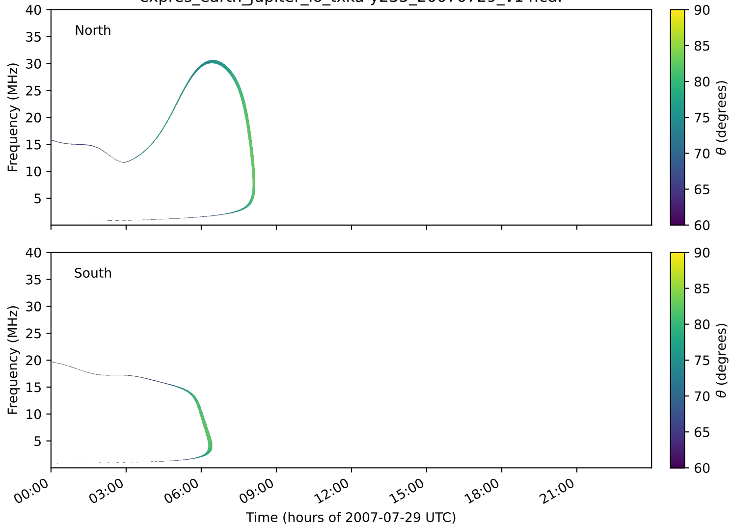
expres_earth_jupiter_io_txka-y235_20070729_v14.cdf
