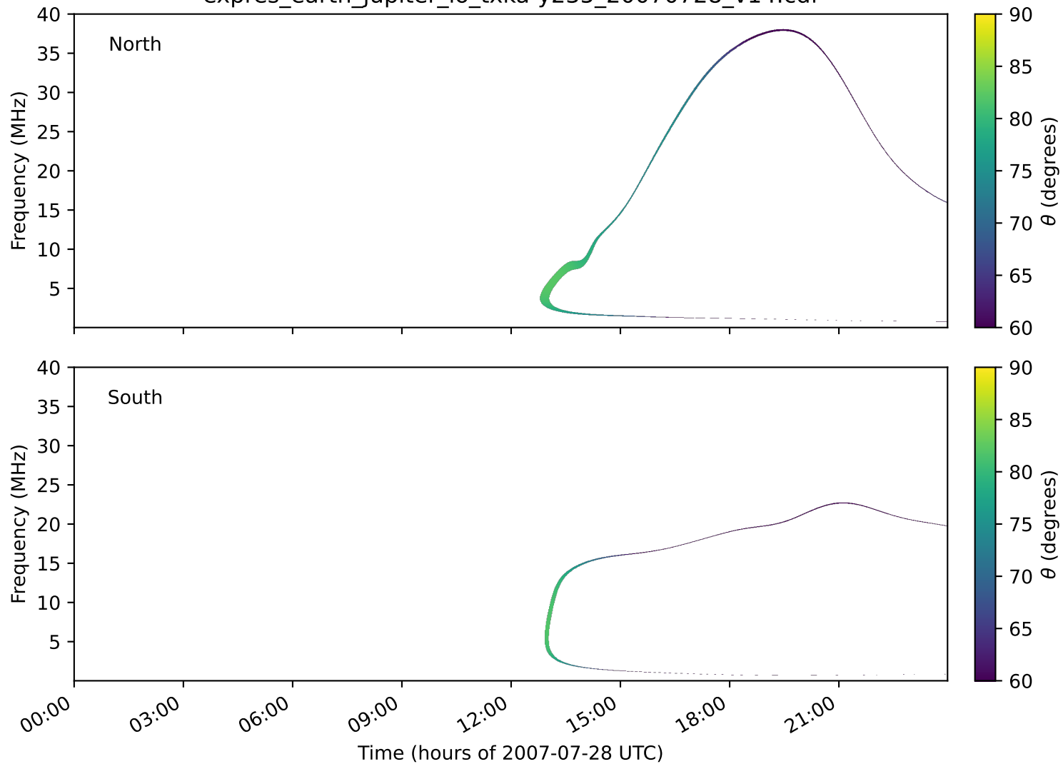
expres_earth_jupiter_io_txka-y235_20070728_v14.cdf
