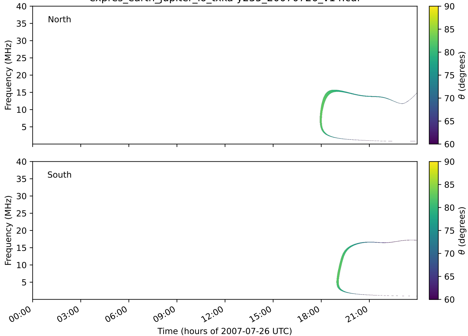
expres_earth_jupiter_io_txka-y235_20070726_v14.cdf
