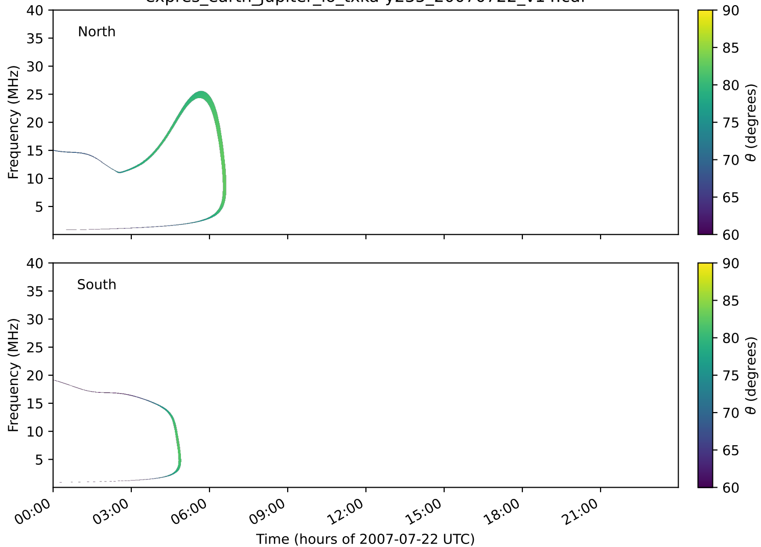
expres_earth_jupiter_io_txka-y235_20070722_v14.cdf
