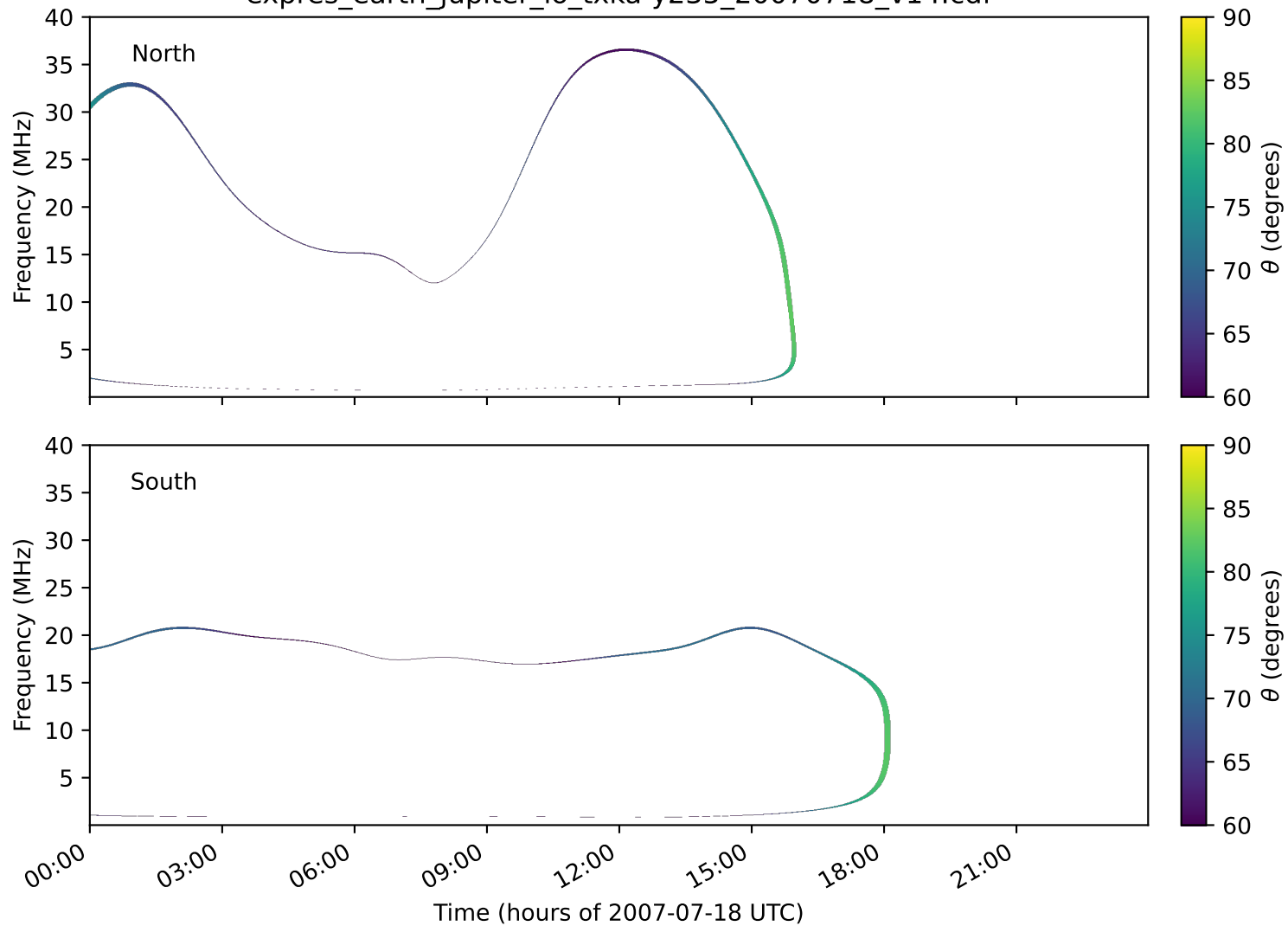
expres_earth_jupiter_io_txka-y235_20070718_v14.cdf
