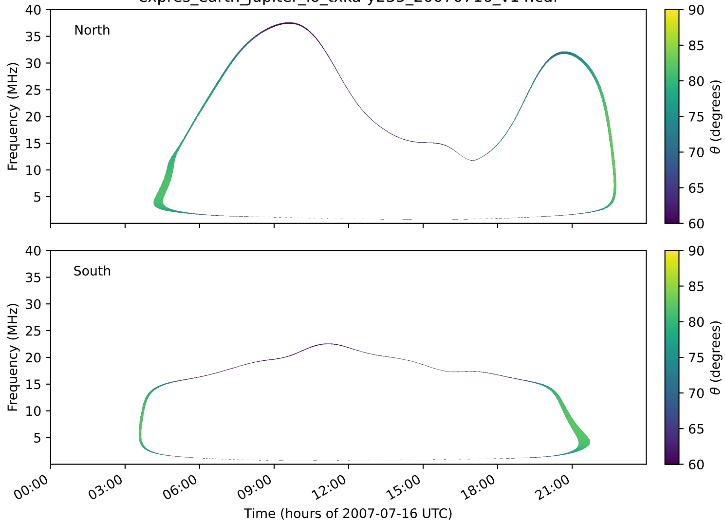
expres_earth_jupiter_io_txka-y235_20070716_v14.cdf
