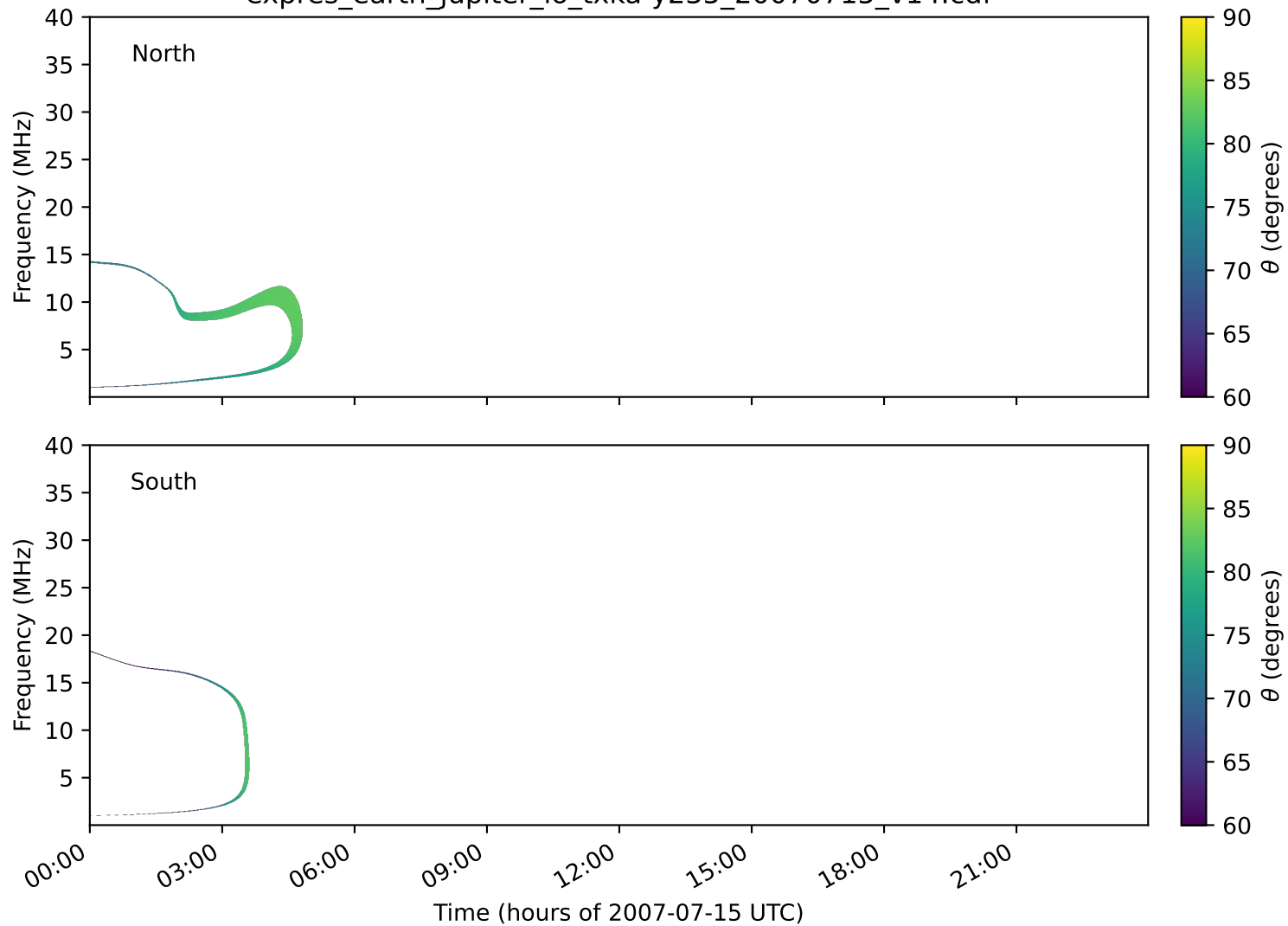
expres_earth_jupiter_io_txka-y235_20070715_v14.cdf
