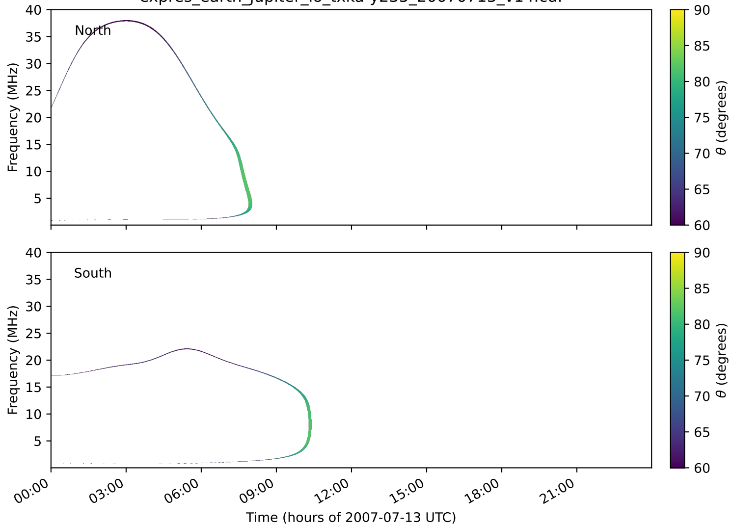
expres_earth_jupiter_io_txka-y235_20070713_v14.cdf
