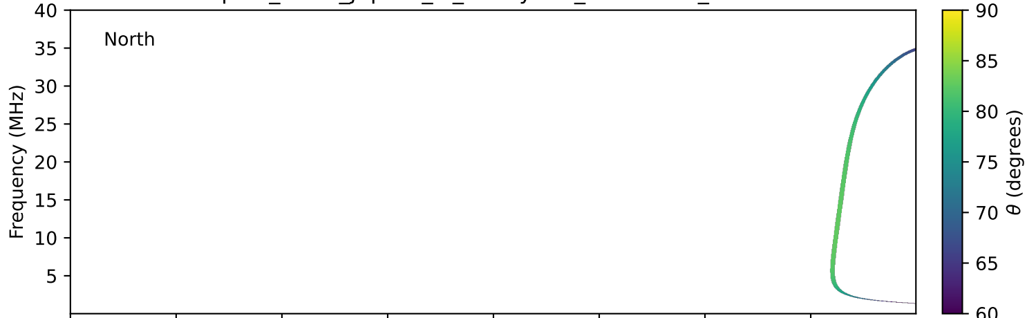
expres_earth_jupiter_io_txka-y235_20070710_v14.cdf
