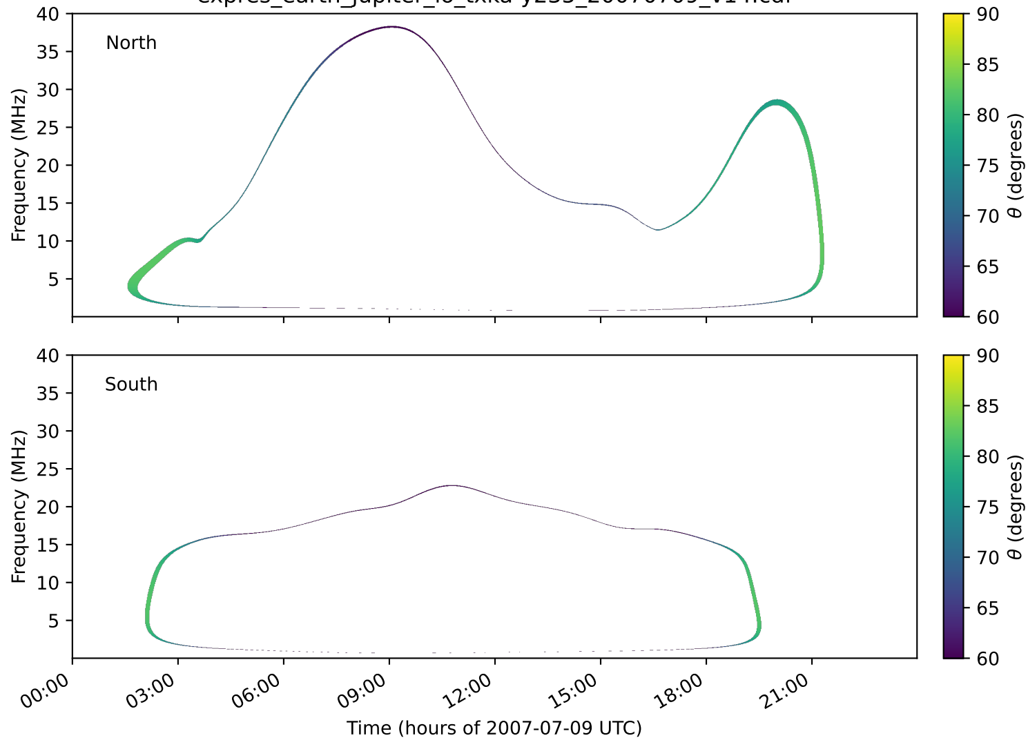
expres_earth_jupiter_io_txka-y235_20070709_v14.cdf
