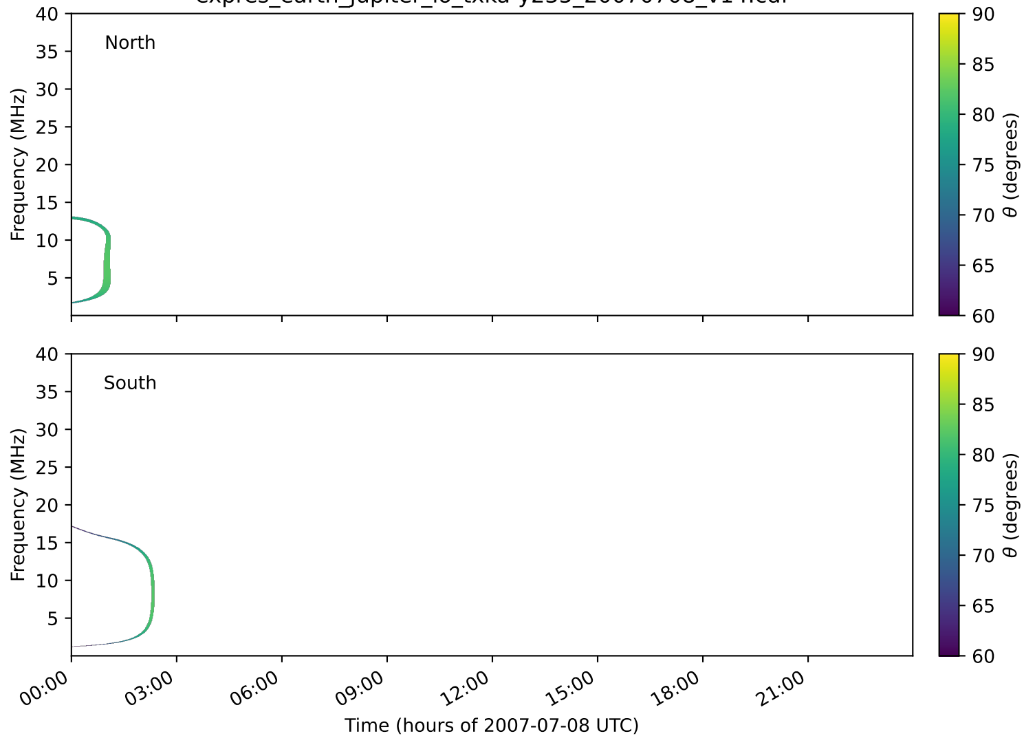
expres_earth_jupiter_io_txka-y235_20070708_v14.cdf
