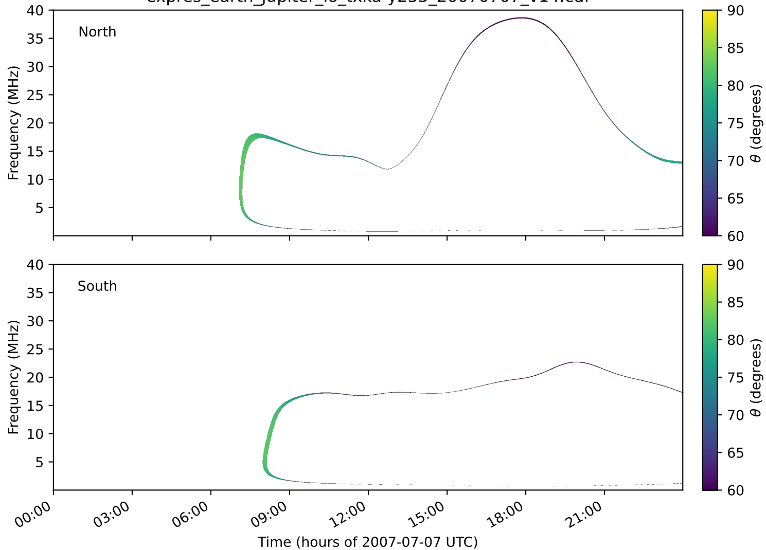
expres_earth_jupiter_io_txka-y235_20070707_v14.cdf
