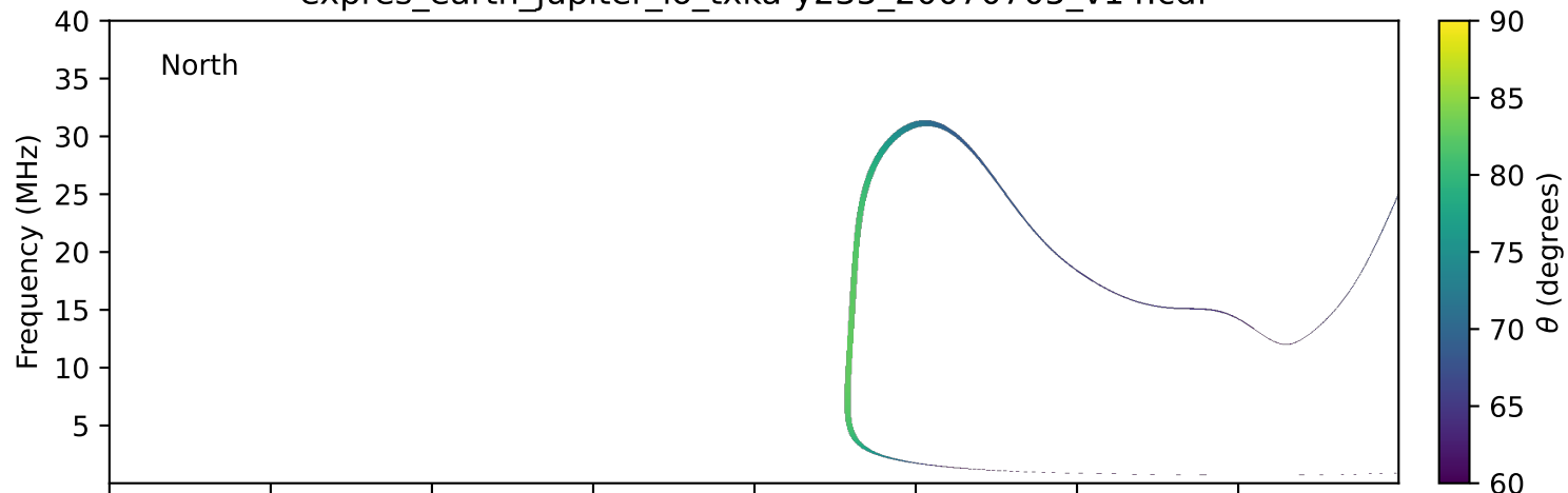
expres_earth_jupiter_io_txka-y235_20070705_v14.cdf
