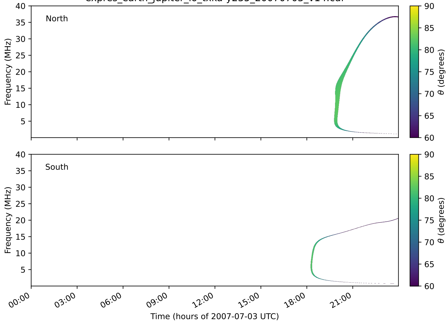
expres_earth_jupiter_io_txka-y235_20070703_v14.cdf
