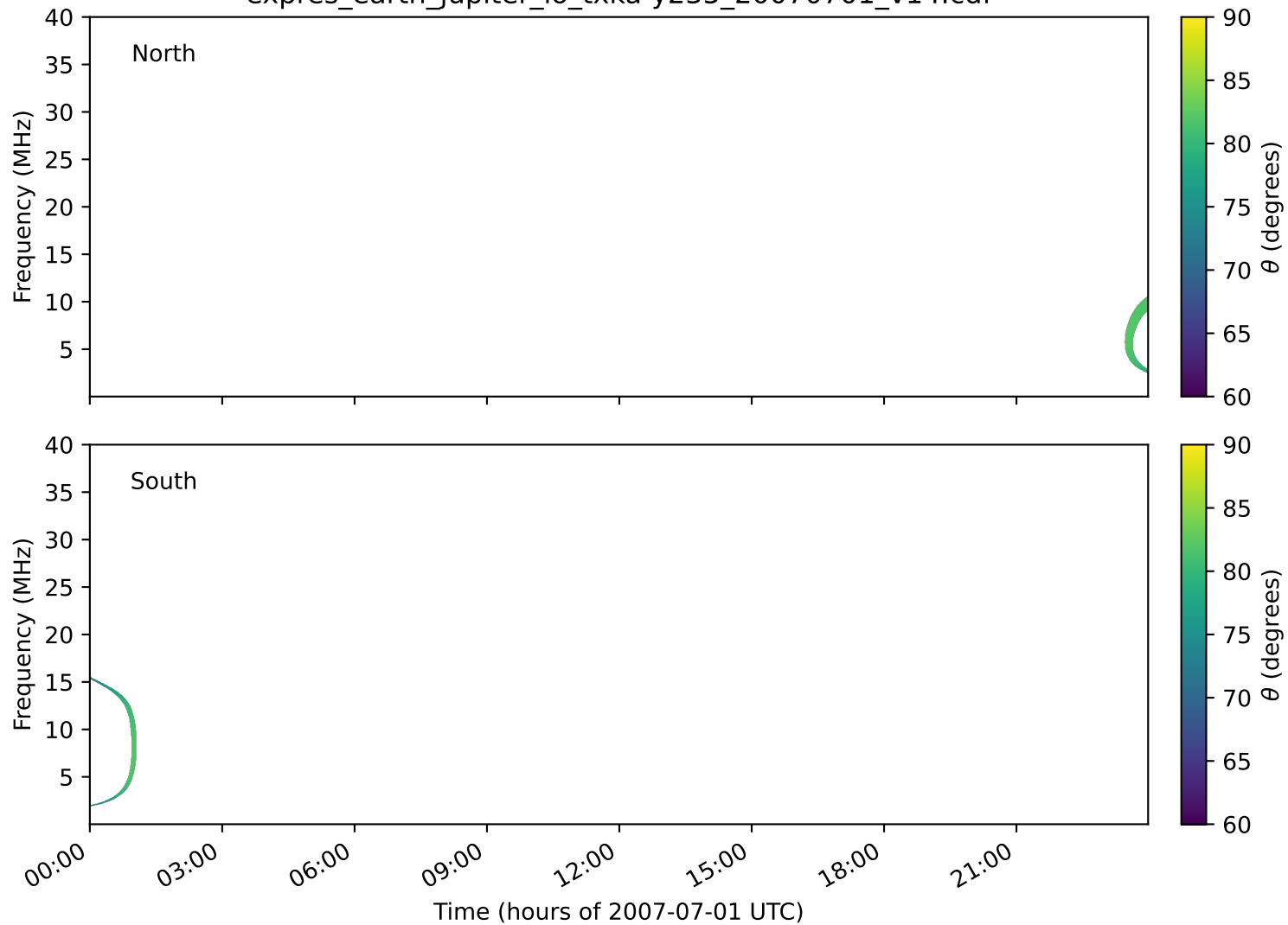
expres_earth_jupiter_io_txka-y235_20070701_v14.cdf
