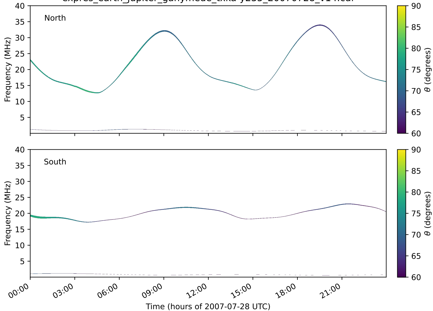
expres_earth_jupiter_ganymede_txka-y235_20070728_v14.cdf
