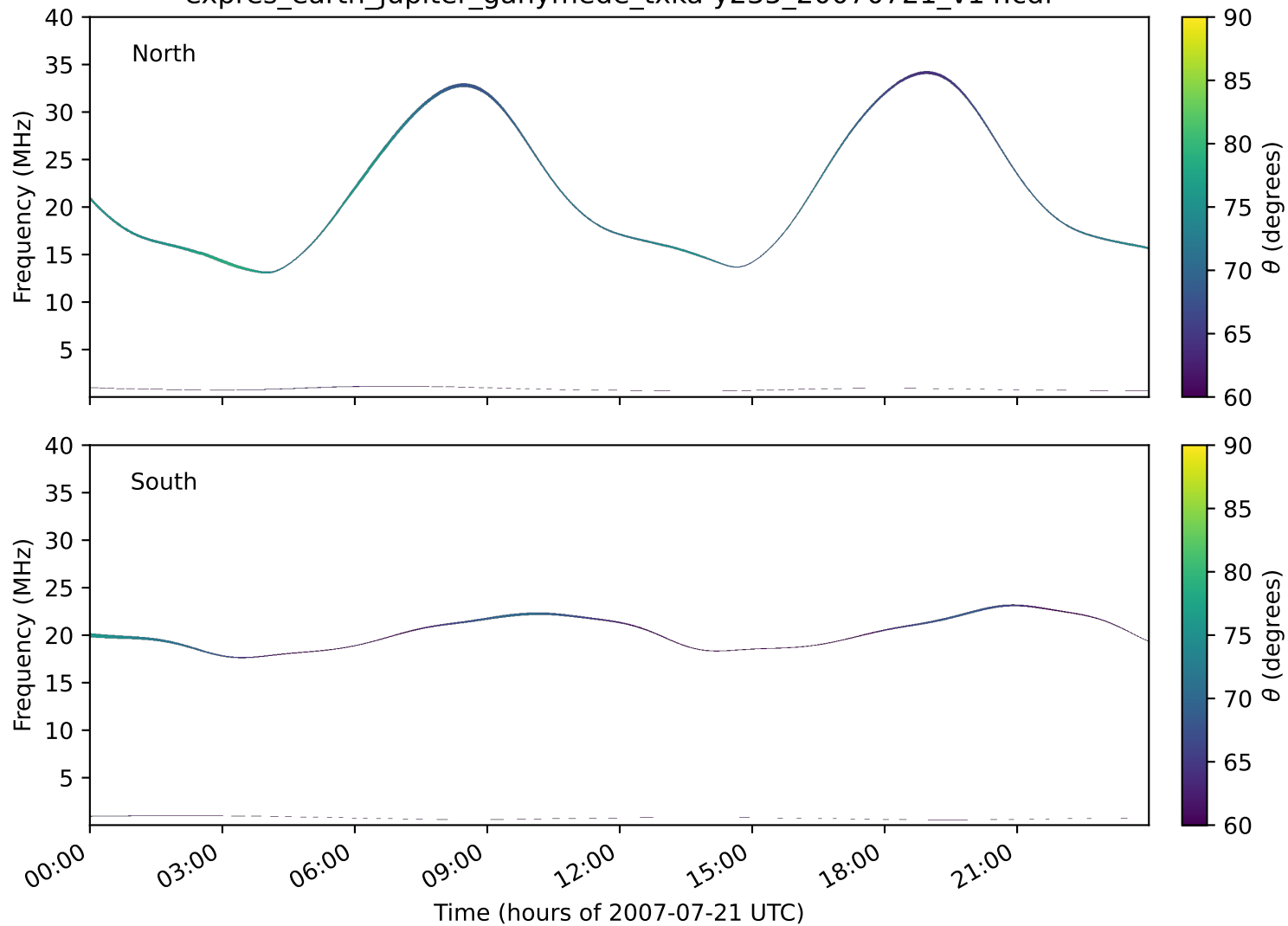
expres_earth_jupiter_ganymede_txka-y235_20070721_v14.cdf
